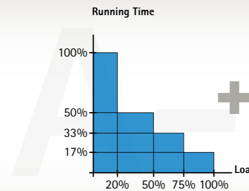
Average capacity utilisation of an industrial crane
