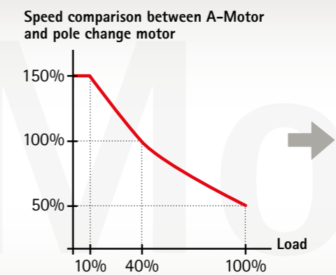
A motor characteristics
